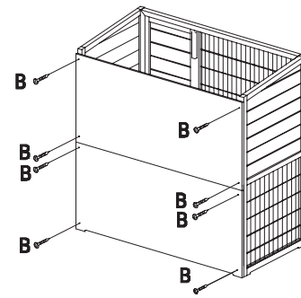
Lid Support
